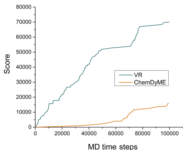
FIG. 5. The time-dependent score as reactions are discovered, using both iMD-VR and the automated ChemDyME software.
