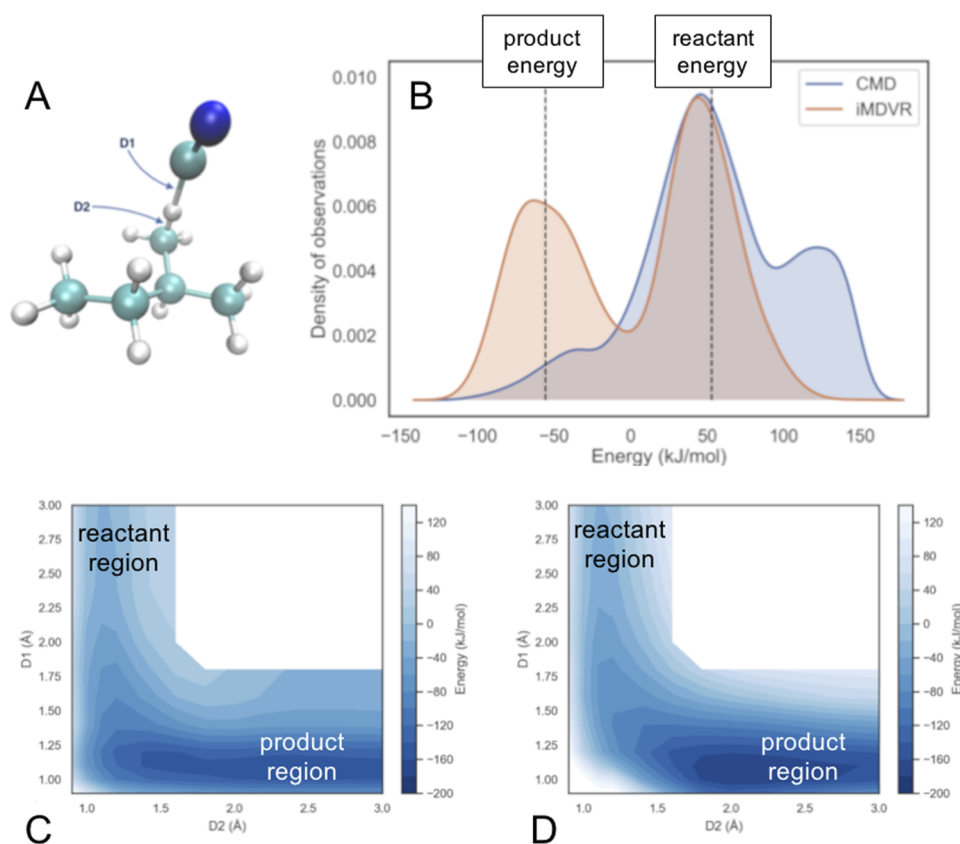
FIG. 3. (a) shows the bond distances defining one particular hydrogen abstraction reaction coordinate for CN + isopentane. (b) shows the kernel density estimate of the configurational energies sampled using the iMD-VR approach (orange) and the constrained MD approach (blue). The dotted lines show the average energy of the sampled reactant and product geometries. Panels (c) and (d) show the PESs predicted by neural nets trained using geometries sampled using iMD-VR and CMD, respectively.
