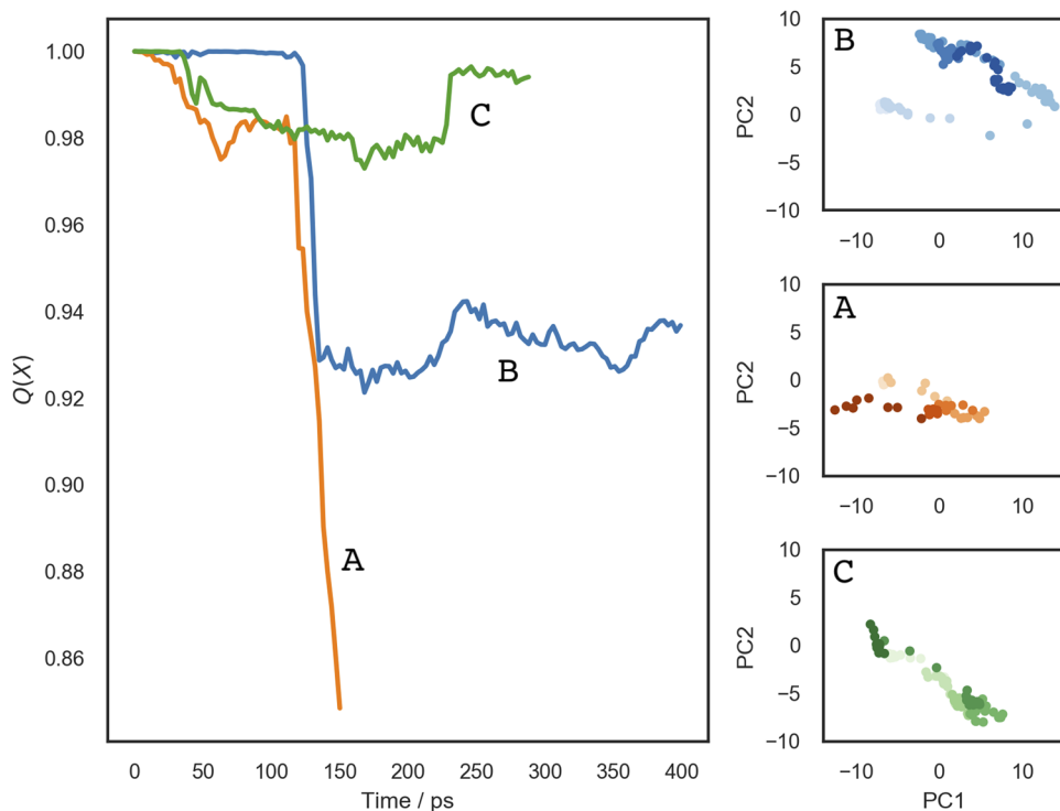
FIG. 7. The left-hand side panel shows fraction of native contacts over the course of the three iMD-VR trajectories (labeled here A, B, and C) in which the 100 s loop motion of CypA was explored; right-hand side panels show the corresponding iMD-VR trajectories projected onto the first two principal components obtained from PCA using the all heavy-atom contact distances as the features. Trajectories are colored from light to dark to indicate the passage of time.
