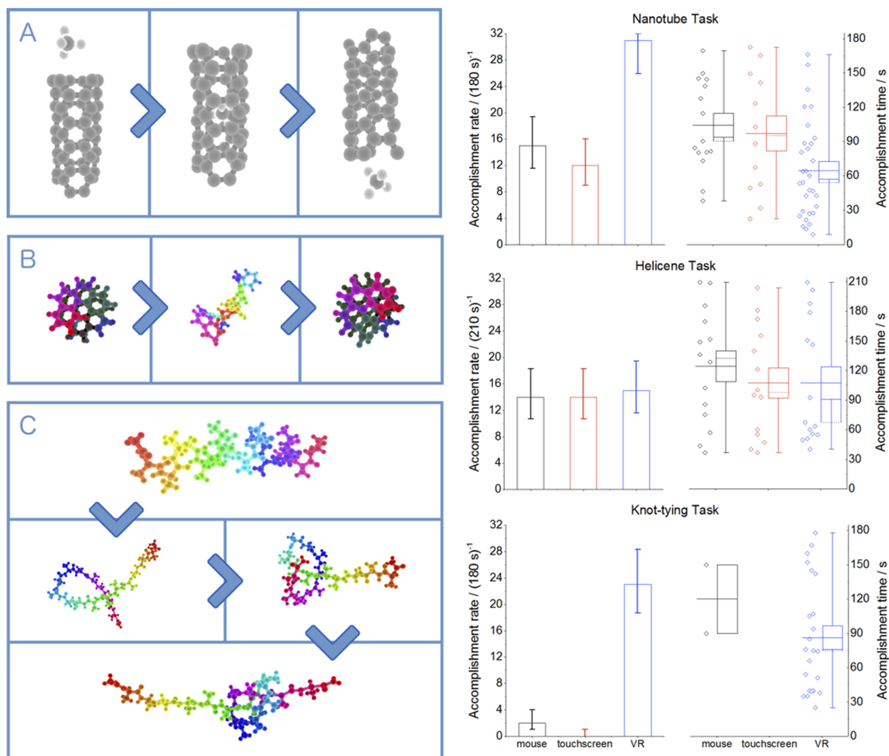
FIG. 2. Left-hand side panels show interactive molecular simulation tasks used as application tests: (a) threading \text{CH}_4 through a nanotube; (b) changing the screw-sense of a helix molecule; and (c) tying a knot in a polypeptide (17-ALA). Colors selected in this figure are chosen for the sake of clarity. The right-hand side panels show the user study results corresponding to each task, including accomplishment rates for each task ( n = 32 for all tasks), with Poisson error estimates, and the distribution of task accomplishment times. In the box-and-whisker plots, whiskers indicate the data range and the box indicates the standard error of the distribution. The mean is shown as a solid line, and the median is shown as a dashed line. Reprinted with permission from M. O'Connor et al. , Sci. Adv. 4 , eaat2731 (2018). 8 Copyright 2018 Author(s), licensed under a Creative Commons Attribution 4.0 License.
