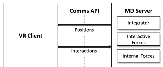
SCHEME 1. Broad outline of the Narupa server/client design and the API that enables communication between the VR client and the MD server. The MD server contains the (thermostated) integrator, as well as engines for calculating both internal and external forces. The API enables flexibility for connecting different force engines to the VR client.
