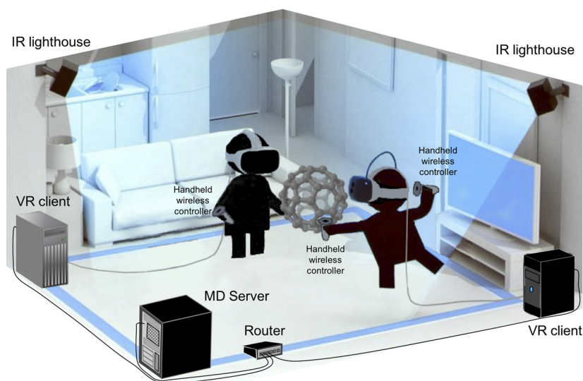
FIG. 1. Schematic of the setup for Narupa, our open-source multiperson iMD-VR framework, showing two participants using handheld wireless controllers to manipulate a real-time MD simulation of a C_{60} molecule. The position of each user's head mounted display (HMD) and wireless controllers is determined using a real-time optical tracking system composed of synchronized IR light sources (“lighthouses”). Each user's HMD is rendered locally on a VR client computer fitted with a suitable graphical processing unit (GPU). MD calculations and maintenance of global user position data take place on a separate MD server, shown here as a local workstation (which alternatively can be cloud-mounted). As long as the network connecting client and server enables sufficiently fast data transfer, system latency is imperceptible. The figure shows a local network setup optimized to minimize latency, with the MD server and VR clients communicating via local area network (LAN) cables connected to a router.
