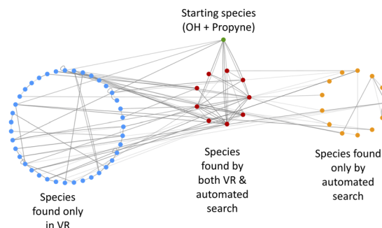
FIG. 4. Comparison of reactions (edges) and species (nodes) found by humans in iMD-VR vs those from the automated ChemDyME software. The starting node (OH + propyne) is green, those chemical species found in both iMD-VR and ChemDyME are in red, those found in iMD-VR only are in blue, and those found from ChemDyME only are in orange.
